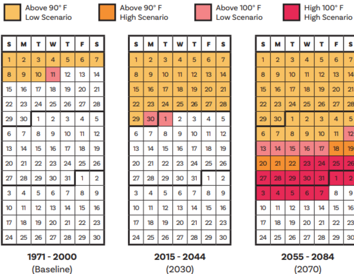
Figure 3-22: Relative increase in projected days above 90°F and 100°F over a three-month period as shown in Cambridge CCVA (City of Cambridge and ATMOS, 2015)
