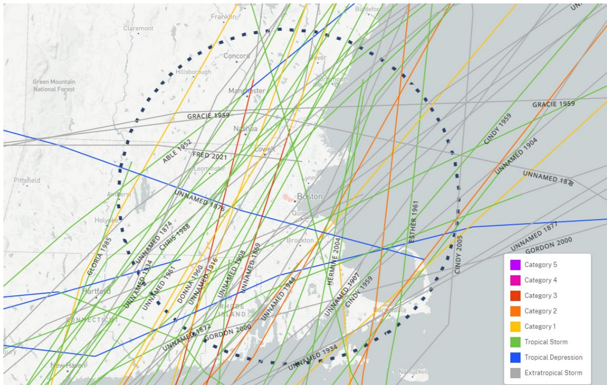
Figure 3-11: Historical Hurricane Tracks followed by storms within 60 nautical miles of Cambridge between 1851 and 2021 (NOAA, 2023)
