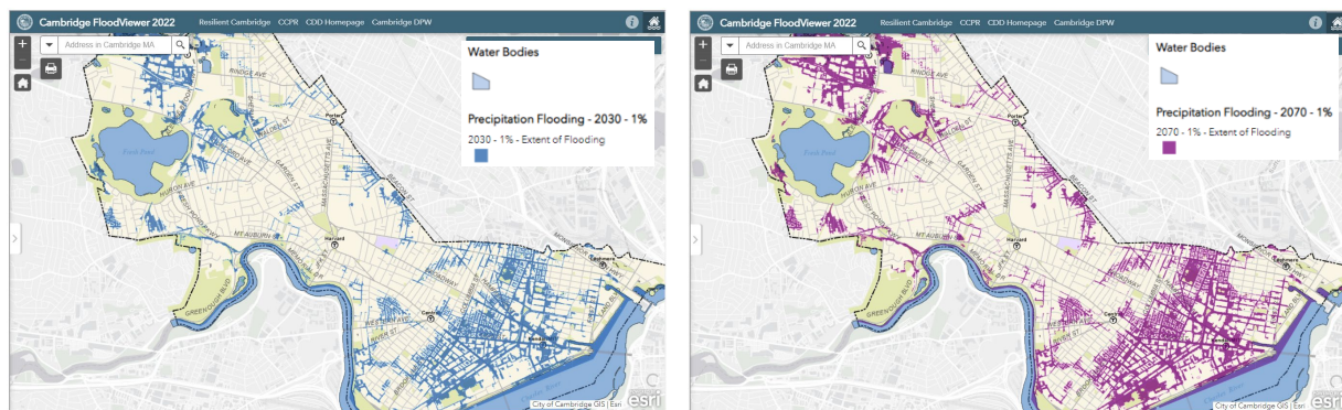
Figure 3-5: Potential flooding from a projected 100-year 24-hour storm with climate change (Left- 2030, Right -2070) and an estimated rainfall of 11.7 inches over 24 hours (Source: Cambridge Flood Viewer)
