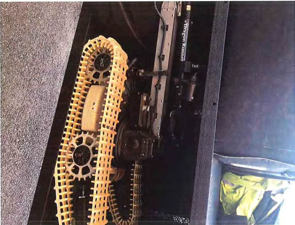
EOD6- Dragon Runner Robot
